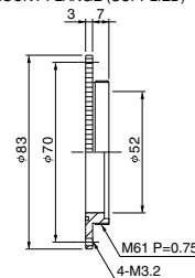
MOUNT FLANGE (SUPPLIED)
