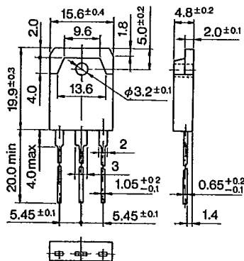
Outline Drawing ⑤
