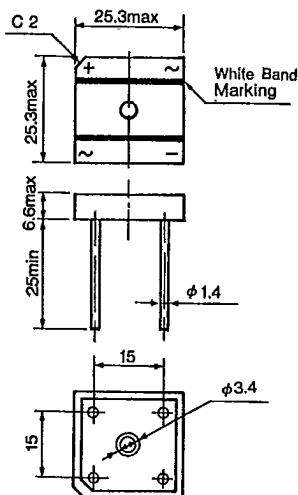
Outline Drawing ⑧
