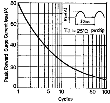
I FSM Characteristics
