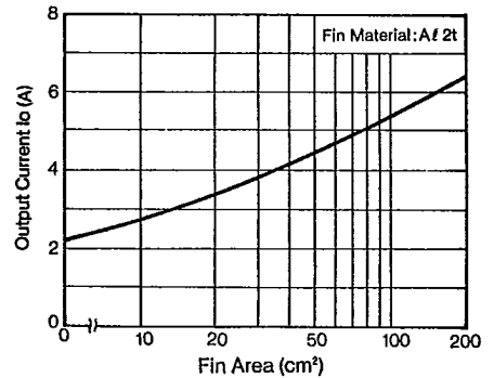
I o - Fin Characteristics
