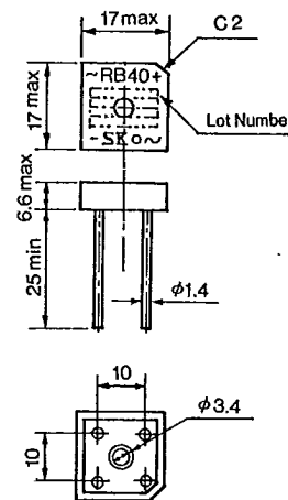
Outline Drawing ⑦
