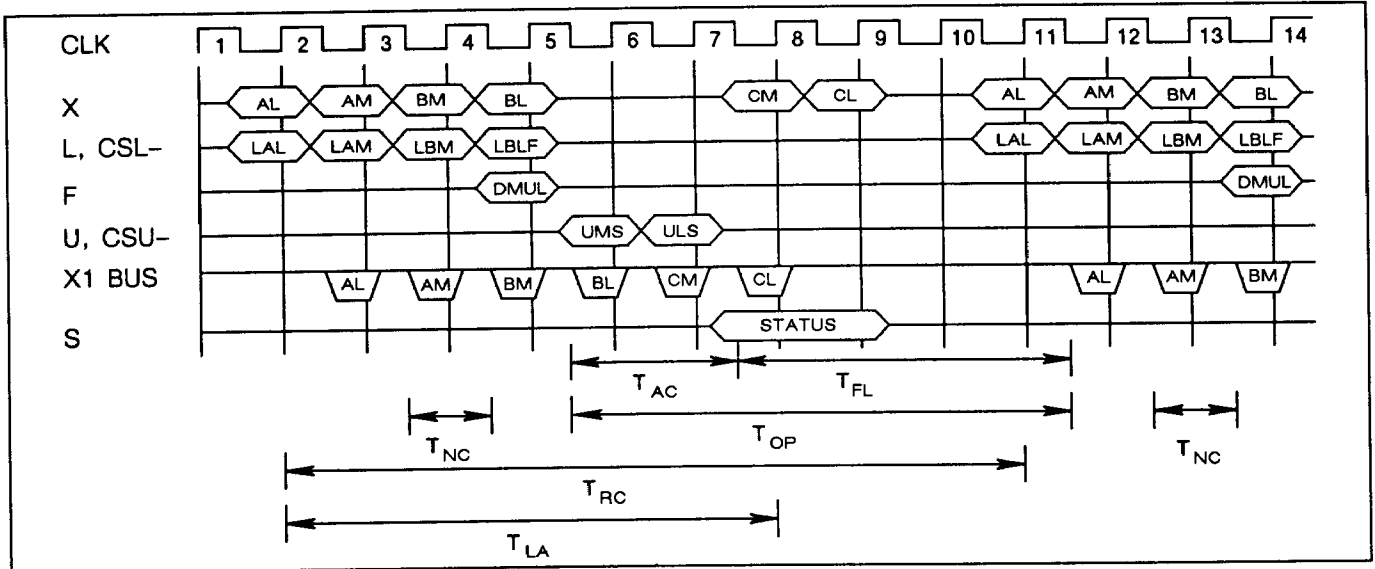
Figure 23. Double Precision Pipelined Multiply
