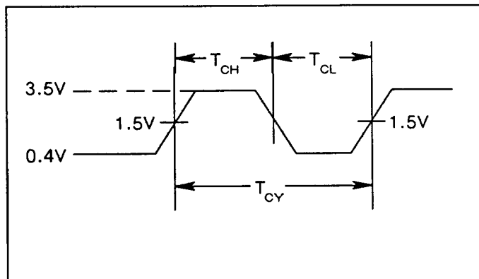
Figure 3. WTL 1164/WTL1165 Clock Timing
