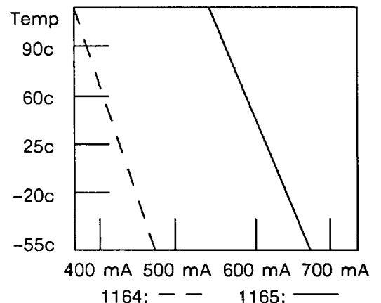
Figure 4. Typical I_{CC} + I_{DD} vs. Temperature
