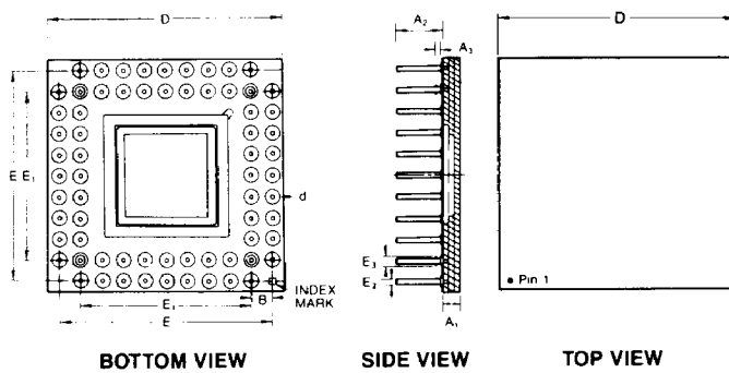
68-PIN PIN GRID ARRAY PACKAGE
