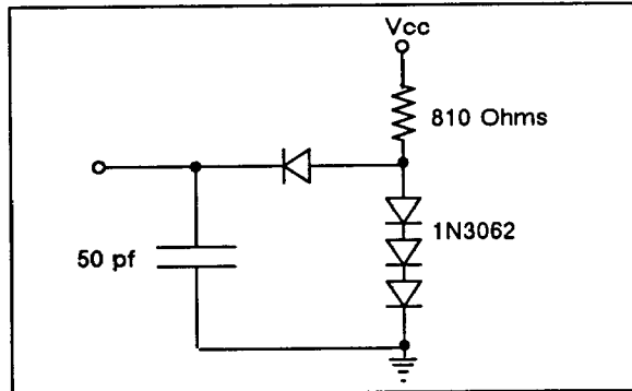
Figure 5. Normal Load Circuit for Delay Measurements
