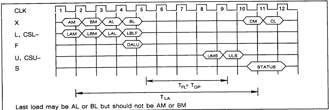
Figure 12. Double Precision ALU Operation
