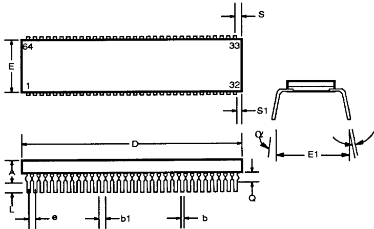
64-PIN DUAL IN-LINE PACKAGE
