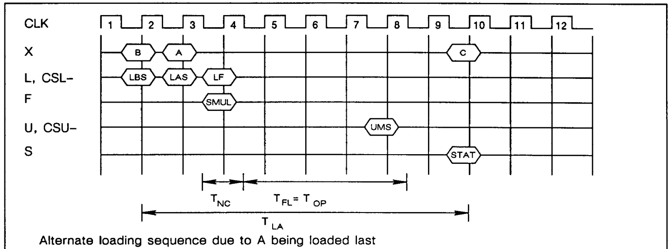
Figure 15. Single Precision Multiply, B Operand First
