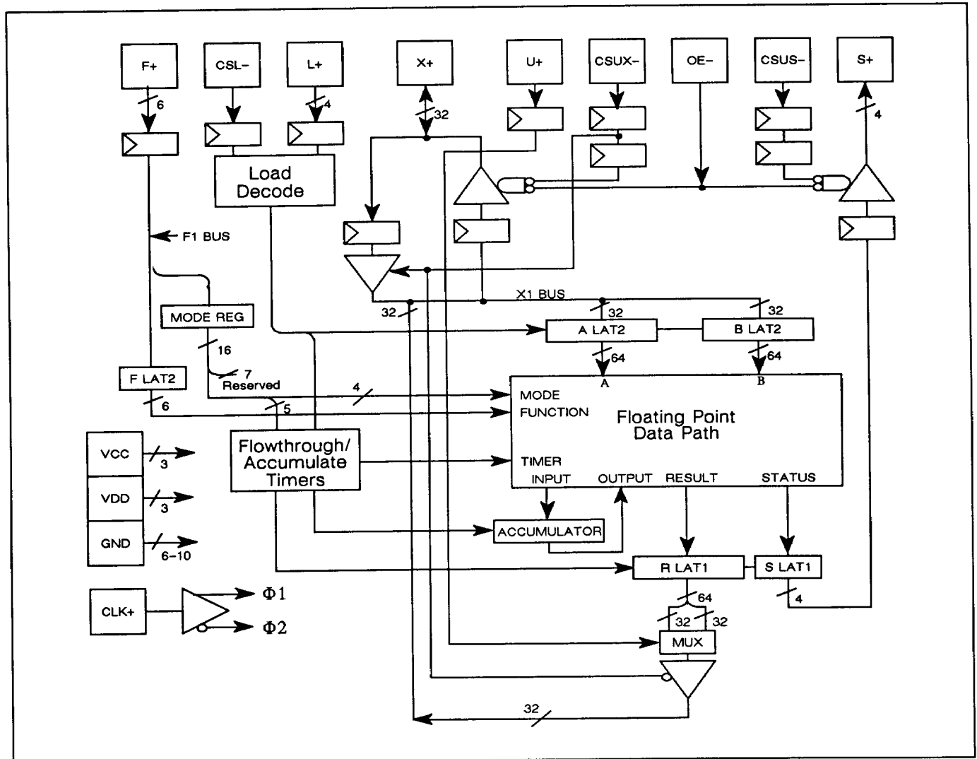
Figure 1. WTL 1164/WTL 1165 Block Diagram
