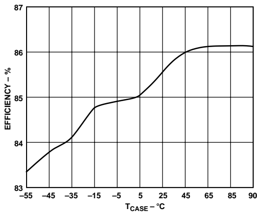
Figure 3. Efficiency vs. Case Temperature (°C) (at Nominal V_{IN} , 75% Max Load, ADC02812DA)
