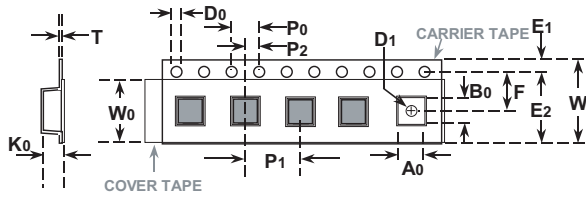
Tape Dimension Items
