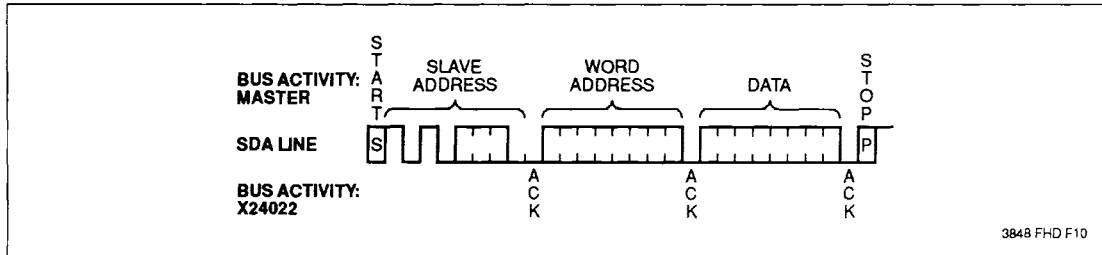
Figure 5. Byte Write
