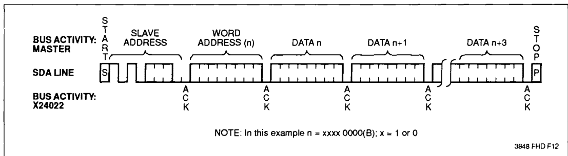
Figure 6. Page Write
