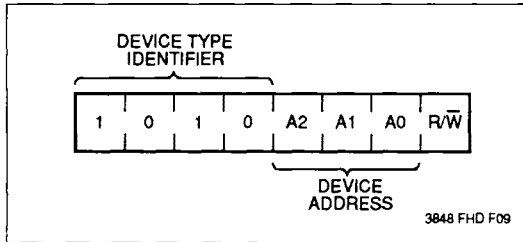
Figure 4. Slave Address
