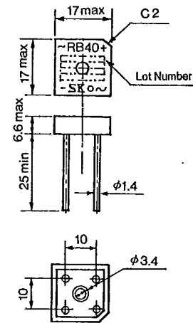
Outline Drawing ⑦
