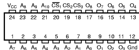
24 Lead Ceramic DIP/24 Lead Sidebraced
