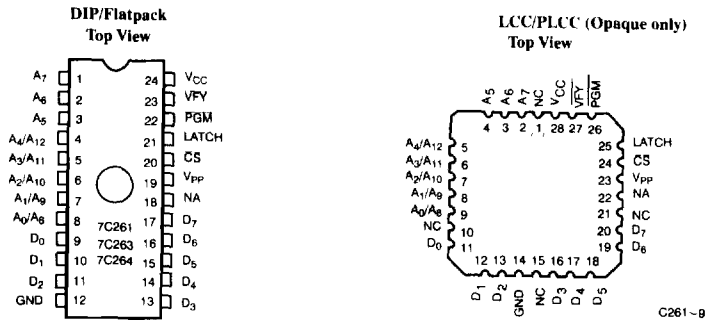
Figure 1. Programming Pinouts
