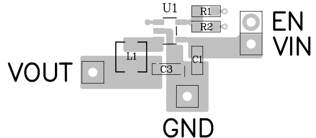
Figure 2—MP28112 Suggested Layout
