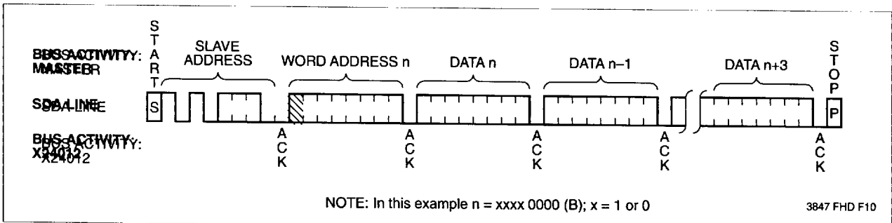
Figure 6. Page Write
