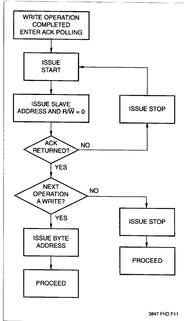
Flow 1. ACK Polling Sequence
