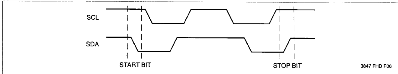
Figure 2. Definition of Start and Stop
