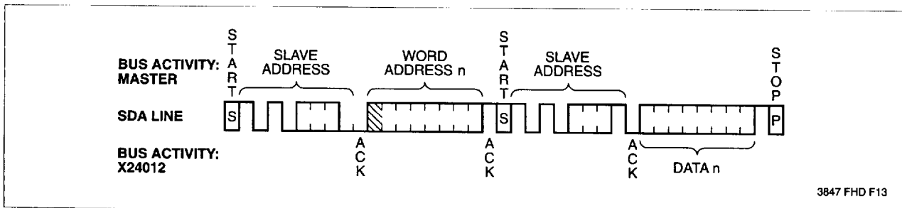
Figure 8. Random Read
