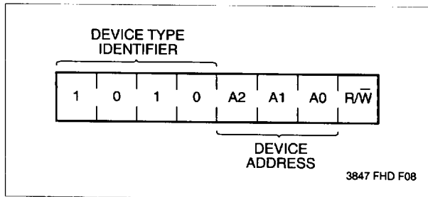
Figure 4. Slave Address
