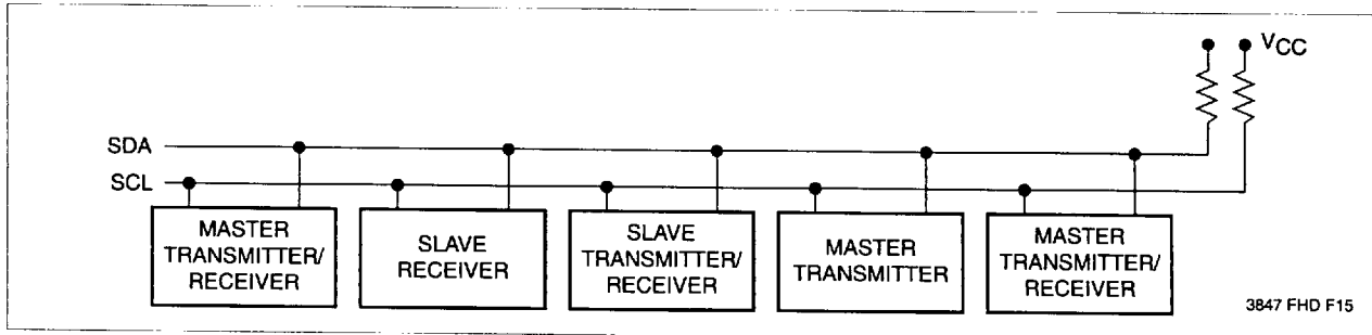
Figure 10. Typical System Configuration
