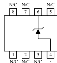
SO-8 SO Package (S)
