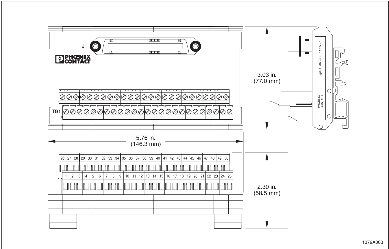
Figure 2. TELCO Dimensions
