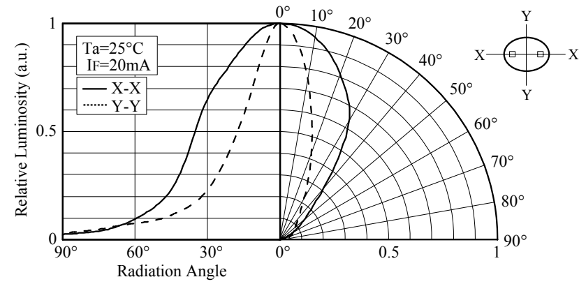
■ Directivity (NSPG636AS)
