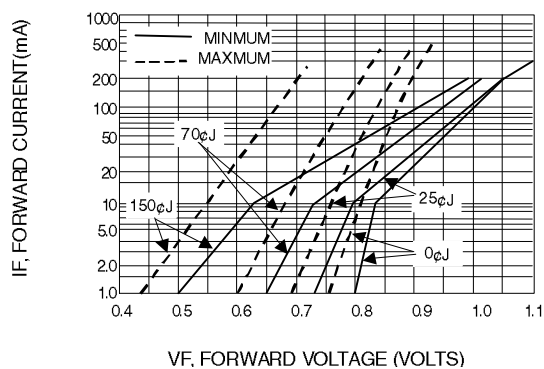
Fig. 10-TYPICAL FORWARD CHARACTERISTICS
