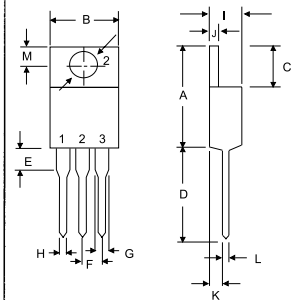
TO-220AB
