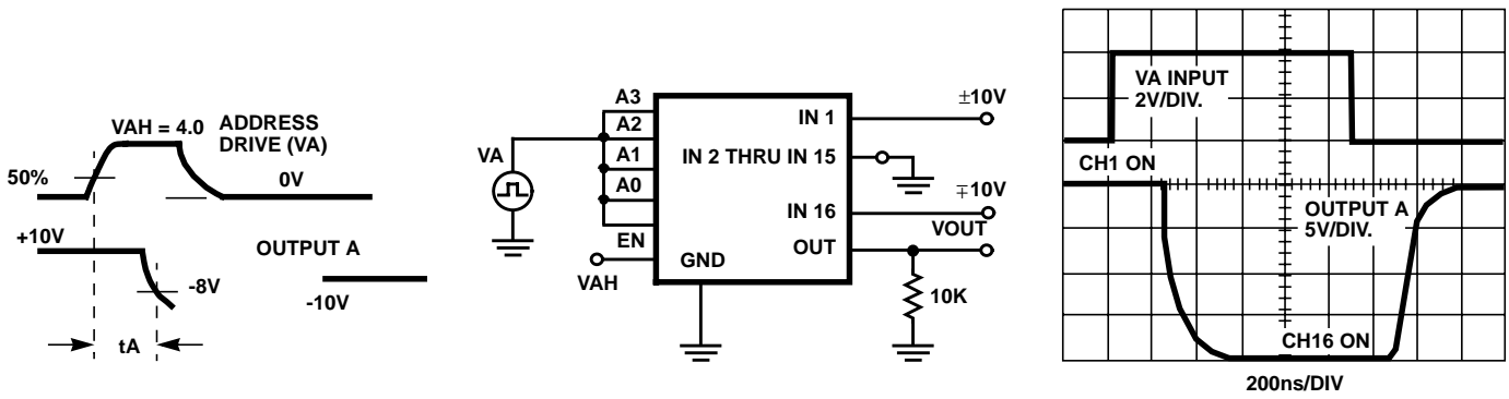
FIGURE 1. ACCESS TIME
