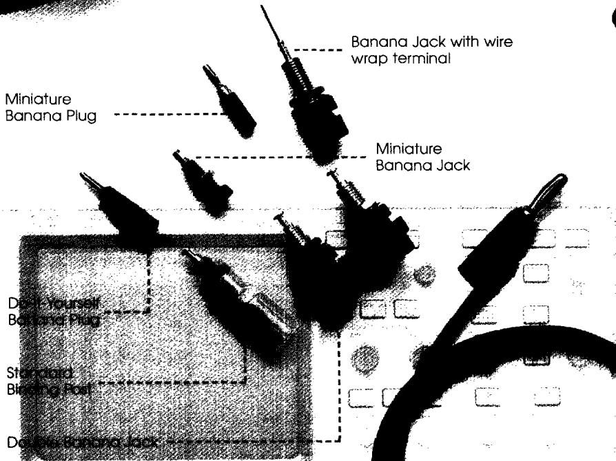
Pomona "B" cords feature 18AWG PVC insulated wire with multiple stacking banana plugs. Nickel-plated beryllium copper springs are swaged in a brass body for best spring retention, low contact resistance and long life. Available in 10 colors, in lengths from 4" to 72". See page 54.
