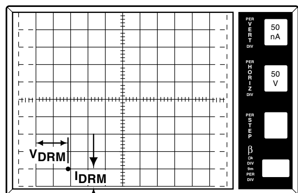
Figure AN1006.22 I_{\text{DRM}} = 50\ \text{nA} at V_{\text{DRM}} = 90\ V
