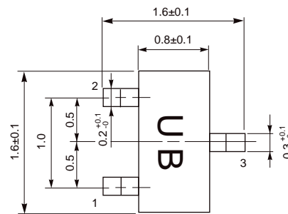
PACKAGE OUTLINE 19
