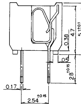
Y-Y' SECTION
