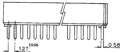
Y-Y' SECTION
