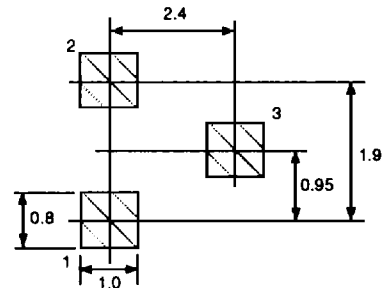
PACKAGE OUTLINE 33 RECOMMENDED P.C.B. LAYOUT
