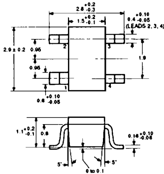
PACKAGE OUTLINE 39
