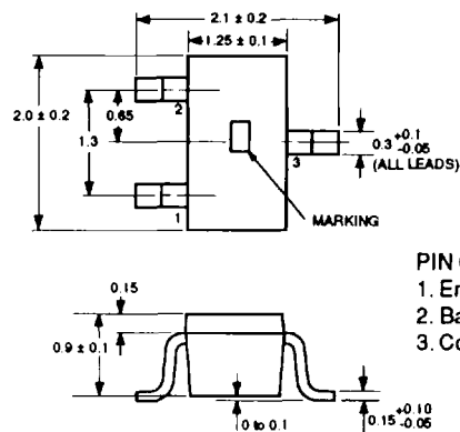
PACKAGE OUTLINE 30
