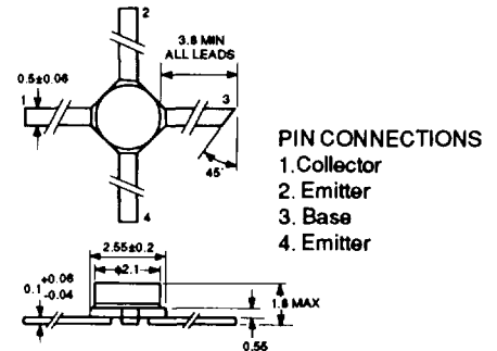
PACKAGE OUTLINE 18 RECOMMENDED P.C.B. LAYOUT
