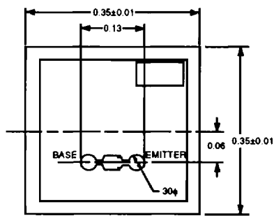
NE68000 (CHIP) (Chip Thickness: 160 μm)
