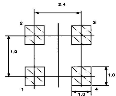
PACKAGE OUTLINE 39 RECOMMENDED P.C.B. LAYOUT
