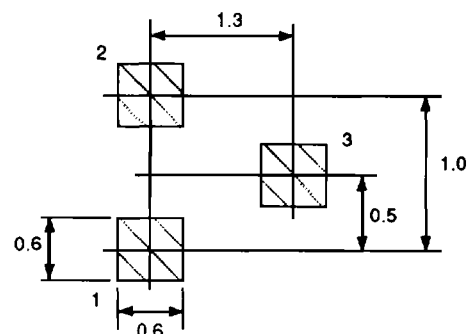
PACKAGE OUTLINE 19 RECOMMENDED P.C.B. LAYOUT
