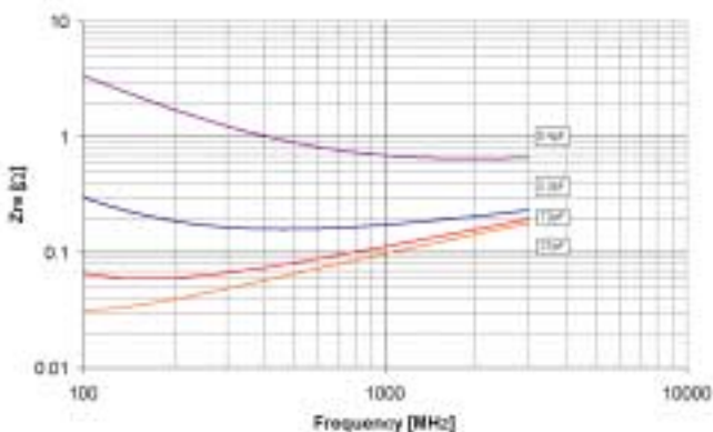
Fig. 5: Typical ESR for different Capacitances vs. Frequency 3
