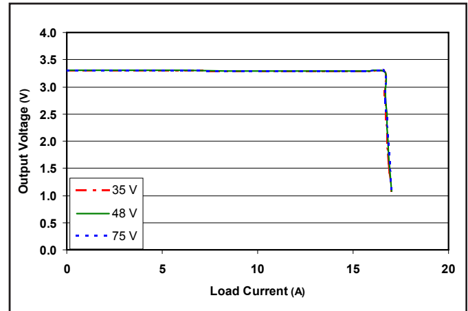
Figure 22: Output voltage vs. load current showing typical current limit curves and converter shutdown points for the 3.3\ \text{V} output. 1.8\ \text{V} load is at 0\ \text{A} .
