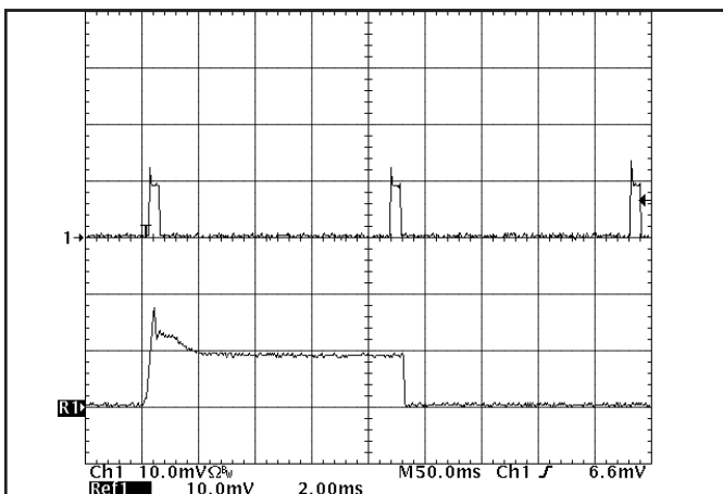
Figure 23: Load current for 1.8\ \text{V} output ( 20\ \text{A}/\text{div} ) as a function of time when the converter attempts to turn on into a 10\ \text{m}\Omega short circuit. Bottom trace is an expansion of the on-time portion of the top trace.
