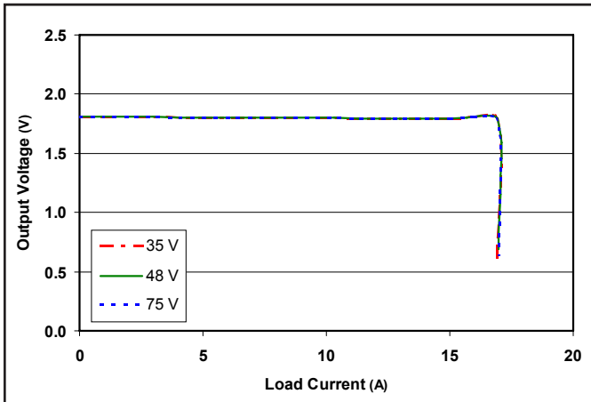
Figure 21: Output voltage vs. load current showing typical current limit curves and converter shutdown points for the 1.8\ \text{V} output. 3.3\ \text{V} load is at 0\ \text{A} .
