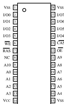
28 TSOP II
