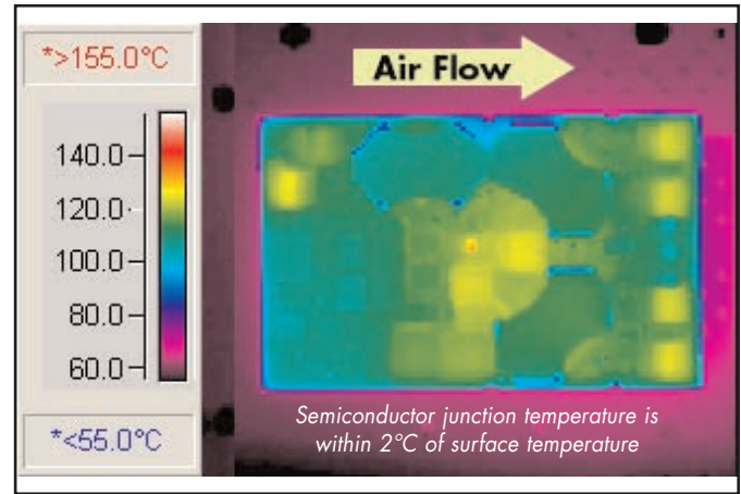
Figure 8: Thermal plot of converter at 23 amp load current with 55°C air flowing at the rate of 200 LFM. Air is flowing across the converter in the long direction from input to output (nominal input voltage).
