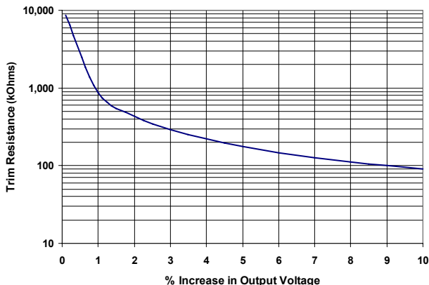
Figure C: Trim Up Graph for 3.3V out
