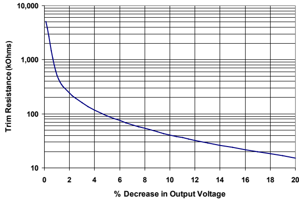
Figure B: Trim Down Graph for 3.3V out
