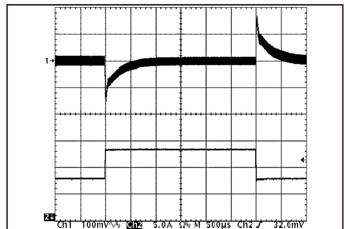
Figure 12: Output voltage response to step-change in load current (50%-75%-50% of I_{max} ; dI/dt = 5A/\mu s ). Load cap: 470 \mu F, 30 m \Omega ESR tantalum capacitor and 1 \mu F ceramic capacitor. Top trace: V_{out} (100mV/div), Bottom trace: I_{out} (5A/div).
