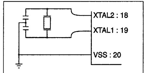
Figure 5 : Crystal Oscillator.
