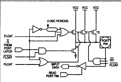
Figure 4 : I/O Buffers in the 83C154 \mu . (Ports 1, 2, 3).
