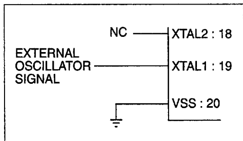
Figure 6 : External Drive Configuration.
