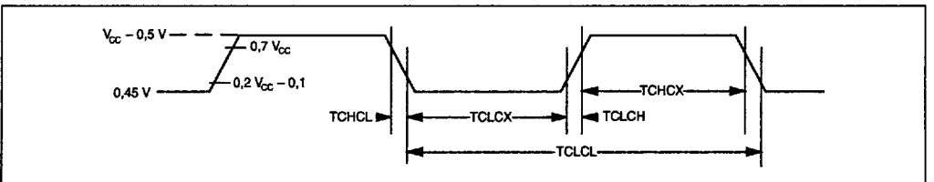
Figure 19 : Clock Signal Waveform for ICC Tests in Actives and Idle Modes. TCLCH = TCHCL = 5 ns.
