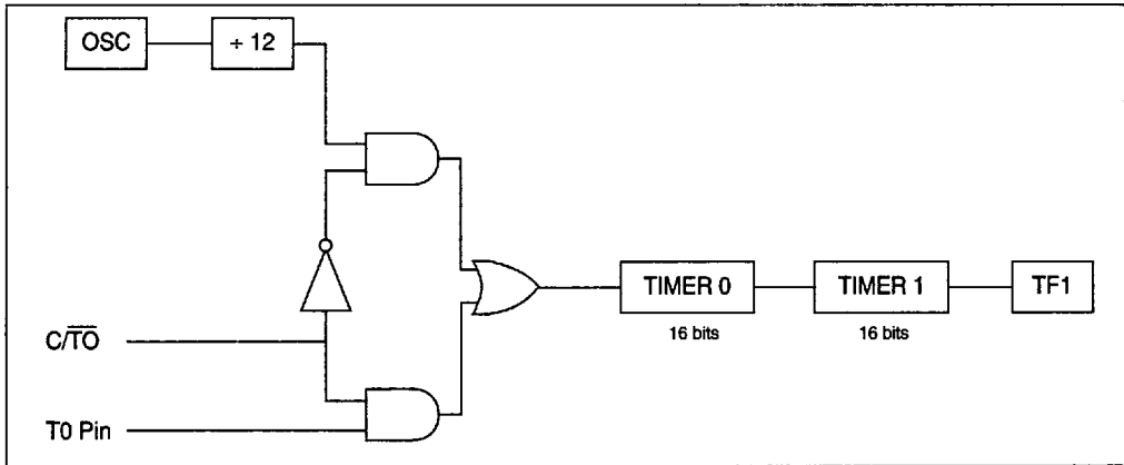
Figure 11 : 32 Bit Timer/counter.
