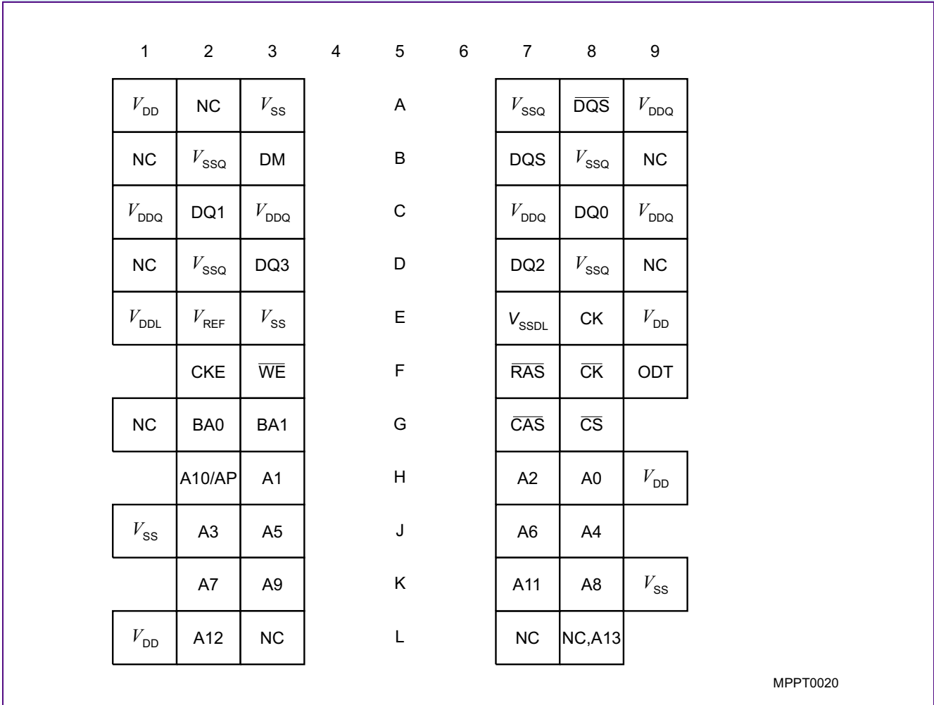
FIGURE 1 Chip Configuration for ×4 components, TFBGA-60 (top view)
