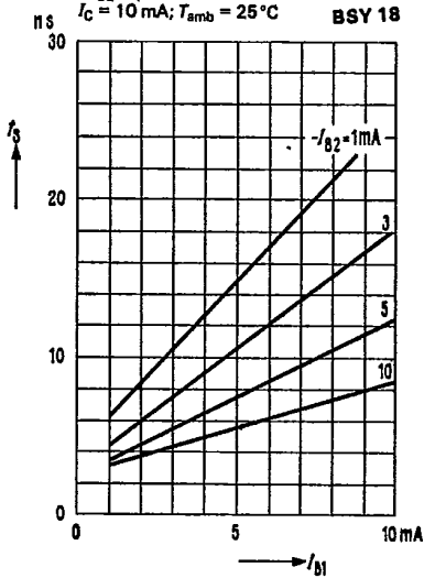
Storage time t_s = f(I_{B1}) -I_{B2} = \text{parameter} I_C = 10 \text{ mA}; T_{amb} = 25^\circ\text{C} BSY 18
