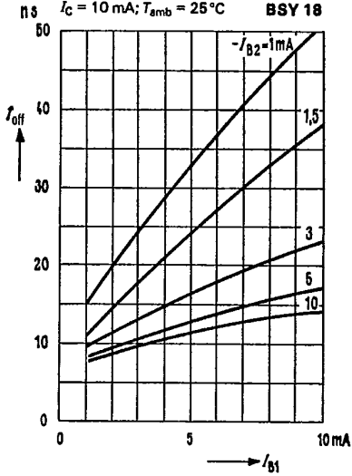
Turn-off time t_{off} = f(I_{B1}) -I_{B2} = \text{parameter} I_C = 10 \text{ mA}; T_{amb} = 25^\circ\text{C} BSY 18
