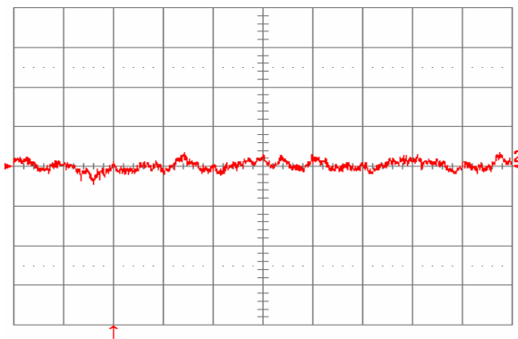
Fig. 25: Input reflected ripple current, i_s (10 mA/div), measured through 10 \mu\text{H} at the source at full rated load current and V_{in} = 24 \text{ V} . Refer to Fig. 23 for test setup. Time scale: 1\mu\text{s}/\text{div} .
