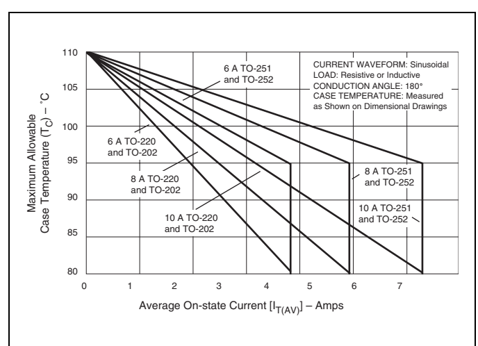
Figure E5.9 Maximum Allowable Case Temperature versus Average On-state Current
