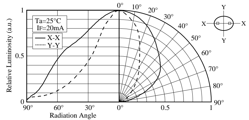
■ Directivity (NSPB346BS)
