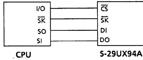
Figure 9 Connectin Example
