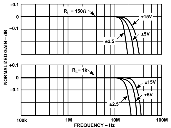
Figure 50. Fine-Scale Gain (Normalized) vs. Frequency for Various Supply Voltages, G = +2 , R_F = 715 \Omega
