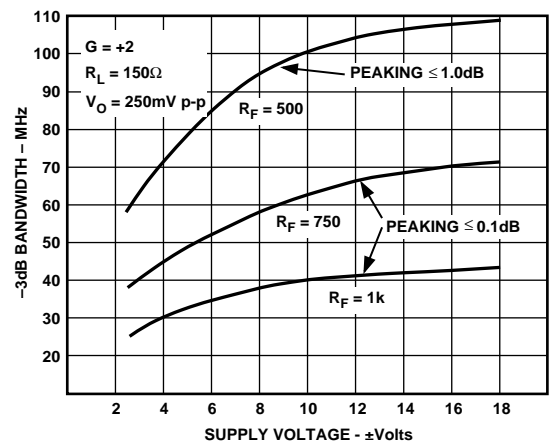
Figure 51. -3 dB Bandwidth vs. Supply Voltage, G = +2 , R_L = 150 \Omega
