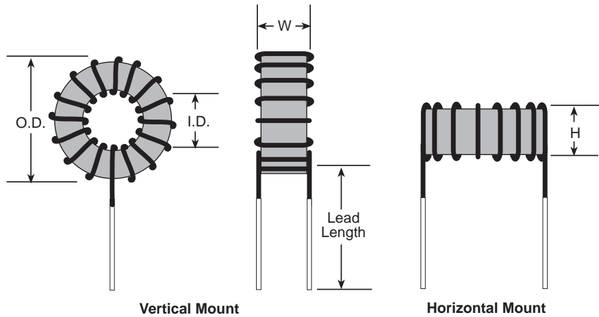
Vertical Mount
