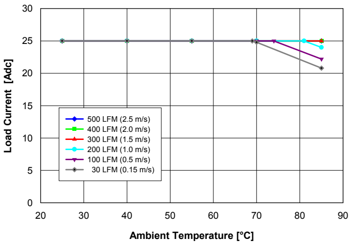
Fig. 1: Available load current vs. ambient air temperature and air-flow rates for Q24S25018 converter mounted vertically with air flowing from pin 3 to pin 1, MOSFET temperature ≤ 120°C, Vin = 27 V.
