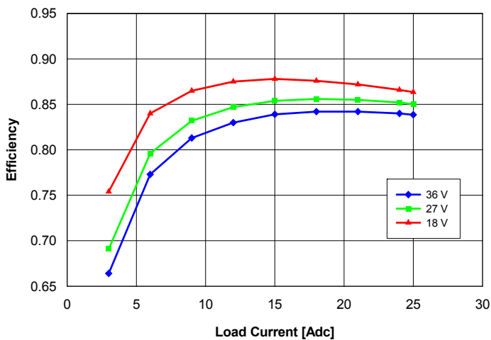
Fig. 16: Efficiency vs. load current and input voltage for converter mounted horizontally with air flowing from pin 3 to pin 4 at a rate of 300 LFM (1.5 m/s) and T_a = 25\text{ }^\circ\text{C} MDC10152 Rev.1.0, 16-Mar-10°C.
