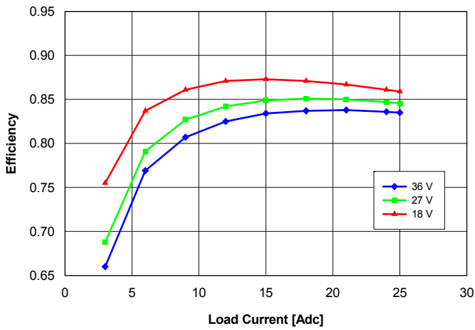
Fig. 14: Efficiency vs. load current and input voltage for converter mounted vertically with air flowing from pin 3 to pin 1 at a rate of 300 LFM (1.5 m/s) and T_a = 25\text{ }^\circ\text{C} .
