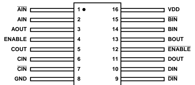
HS9-26C32RH 16 LEAD FLATPACK MIL-STD-1835: CDFP4-F16 TOP VIEW
