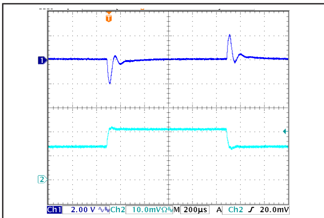
Figure 5: Output voltage response to step-change in load current (50%-75%-50% of I out (max); dI/dt = 0.05 A/µs). Load cap: 1 µF ceramic capacitor. Ch 1: V out (2 V/div), Ch 2: I out (2 A/div).
