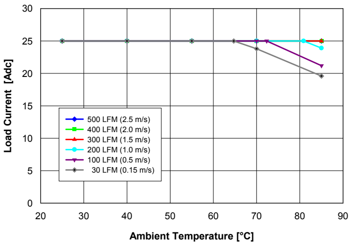
Fig. 1: Available load current vs. ambient air temperature and air-flow rates for Q24T25018 converter mounted vertically with air flowing from pin 3 to pin 1, MOSFET temperature \leq 120^{\circ}\text{C} , V_{in} = 27\text{ V} .
