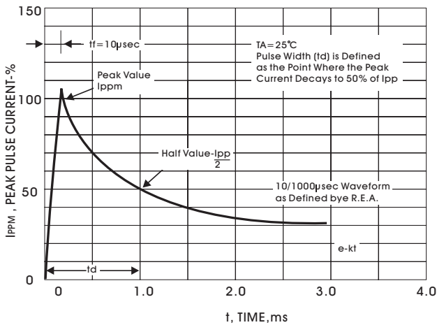
FIGURE 3-PULSE WAVEFORM
