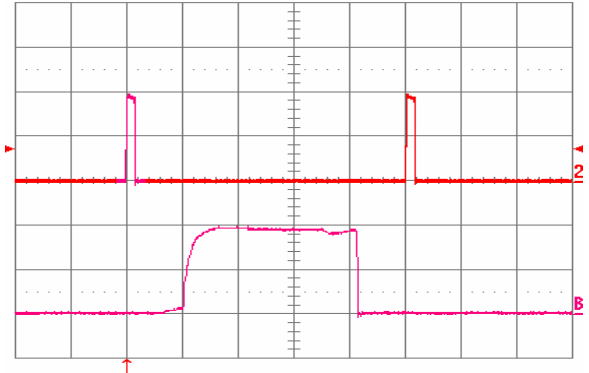
Fig. 27: Load current (top trace, 20 A/div, 20 ms/div) into a 10 m \Omega short circuit during restart, at V_{in} = 48 V. Bottom trace (20 A/div, 1 ms/div) is an expansion of the on-time portion of the top trace.
