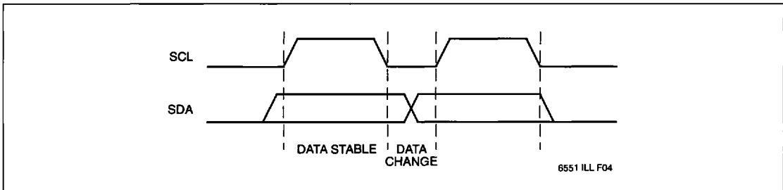
Figure 1. Data Validity
