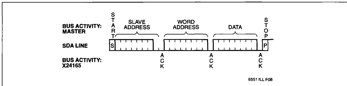
Figure 5. Byte Write
