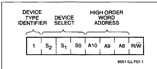
Figure 4. Slave Address
