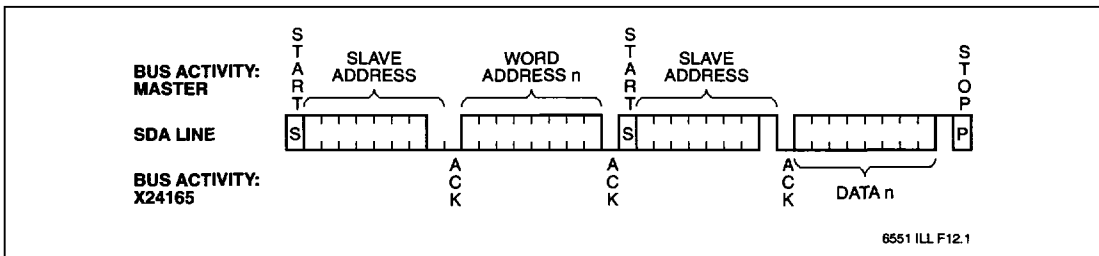
Figure 8. Random Read
