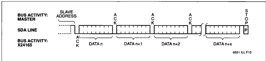
Figure 9. Sequential Read
