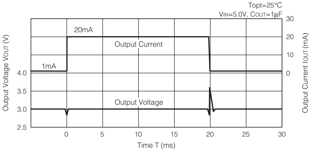
R1150H (VR=5.0V)
