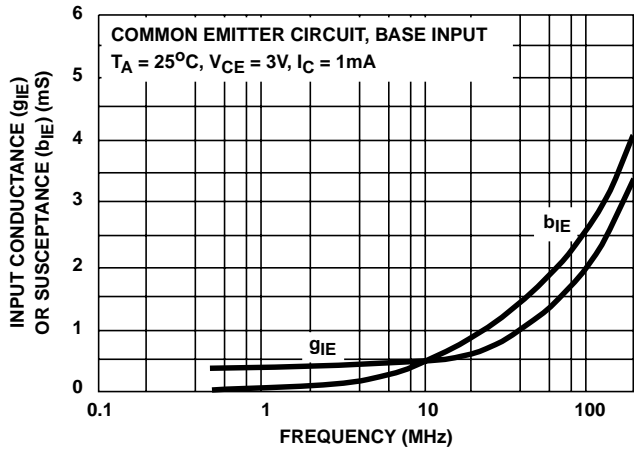
FIGURE 15. INPUT ADMITTANCE ( Y_{IE} )
