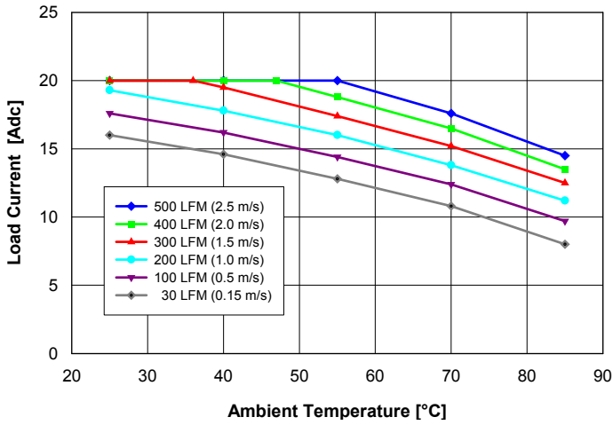
Fig. 10: Available load current vs. ambient air temperature and airflow rates for Q48T20050 converter with D height pins mounted vertically with V_{in} = 48\text{ V} , air flowing from pin 3 to pin 1 and maximum FET temperature \leq 120^{\circ}\text{C} .
