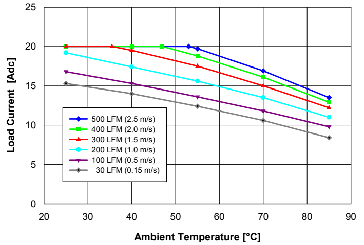
Fig. 11: Available load current vs. ambient air temperature and airflow rates for Q48T20050 converter with D height pins mounted horizontally with V_{in} = 48\text{ V} , air flowing from pin 3 to pin 1 and maximum FET temperature \leq 120^{\circ}\text{C} .
