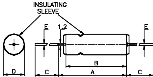
Fig. 7 Case Sizes - Outline and Dimensions
