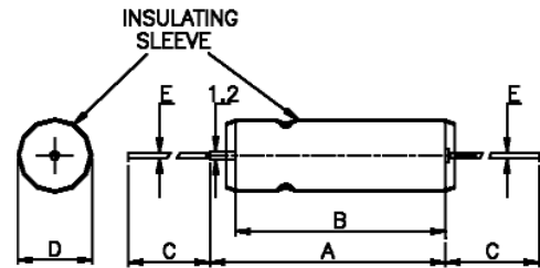
Fig. 1. Case Sizes - Outline and Dimensions
