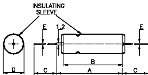
Fig. 4 Case Sizes - Outline and Dimensions
