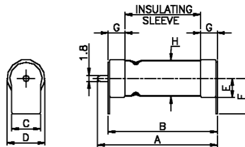
Fig. 8 Case Sizes - Outline and Dimensions
