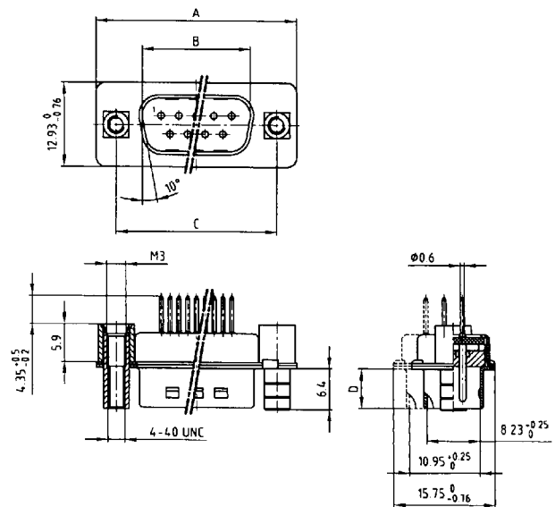
Plug connector
