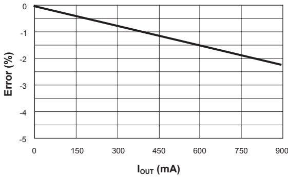
Load Regulation
