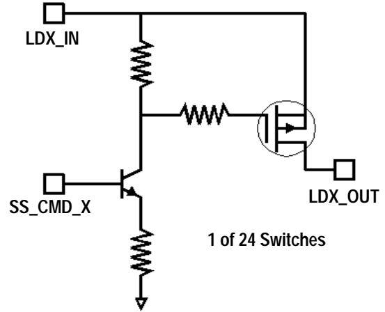
Logic Diagram
