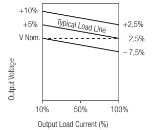
Tolerance Envelope
